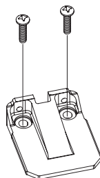
98/99 and 33/35 device mechanism case bracket
