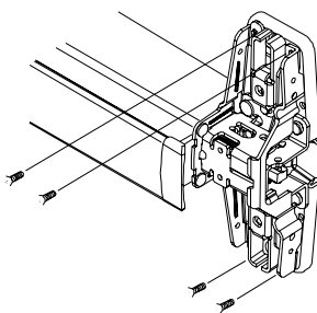
98/9927 center case shown
